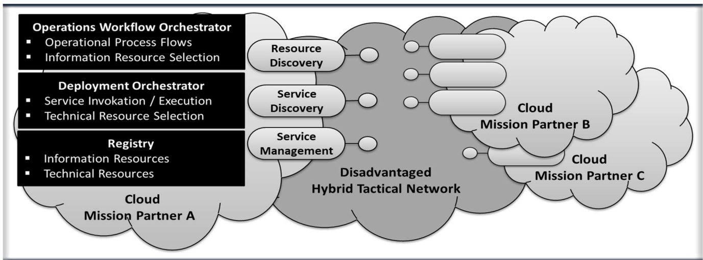
Fig. 1. Artifacts for the federated cloud: service APIs and capabilities.
