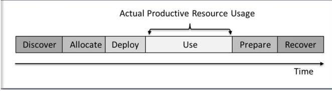
Fig. 3. Resource utilization phases.
