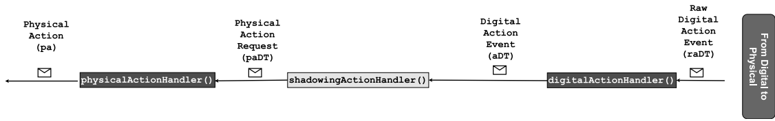
Fig. 6. From DT to PT actions shadowing.
