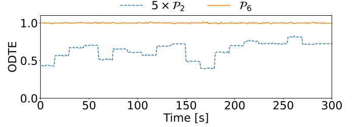
Fig. 5: ODTE comparison: 5 \times \mathcal{P}_2 vs. \mathcal{P}_6 (1 from 5).
