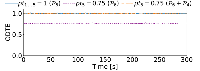
Fig. 6: ODTE degradation of \mathcal{P}_6 with a slower PT ( pt_5 = 0.75 ) and possible countermeasure ( \mathcal{P}_6 + \mathcal{P}_4 ).
