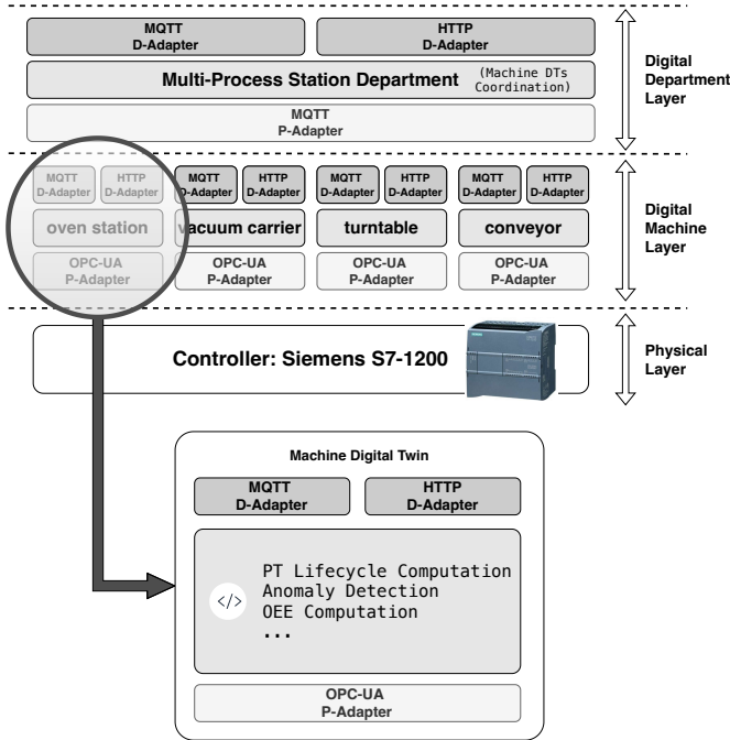
Fig. 5: Multi-process Station Digital Twin overview.
